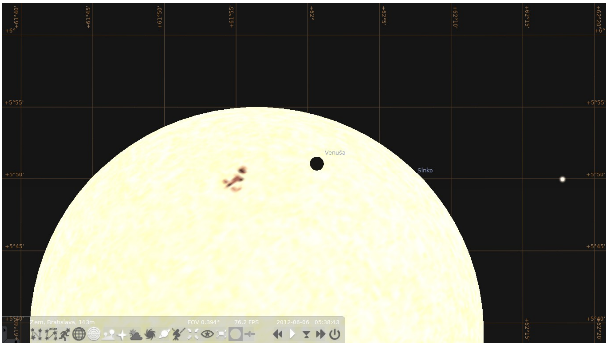
program Stellarium
